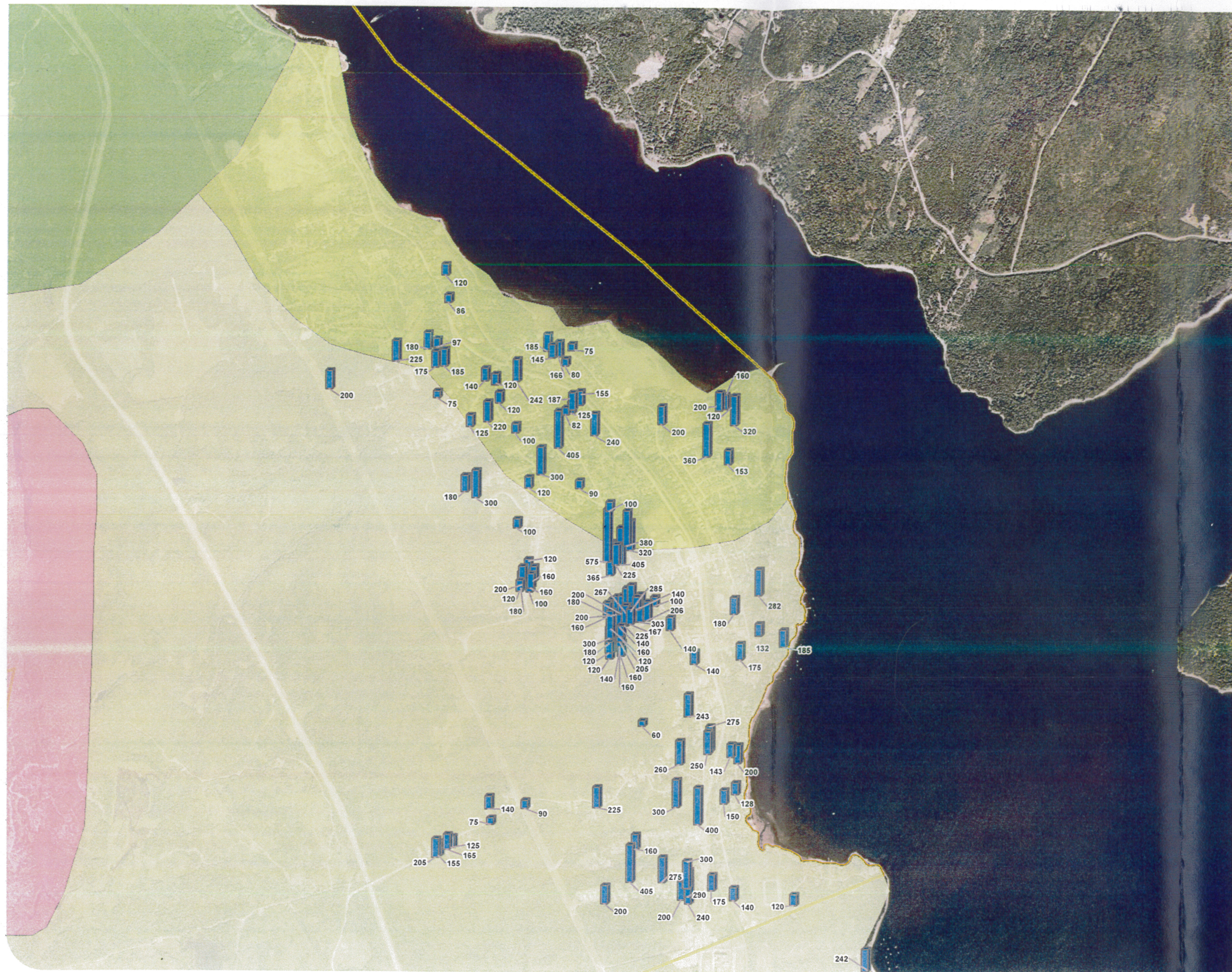
FIGURE 4A SURFICIAL GEOLOGY AND WELL DEPTHS
