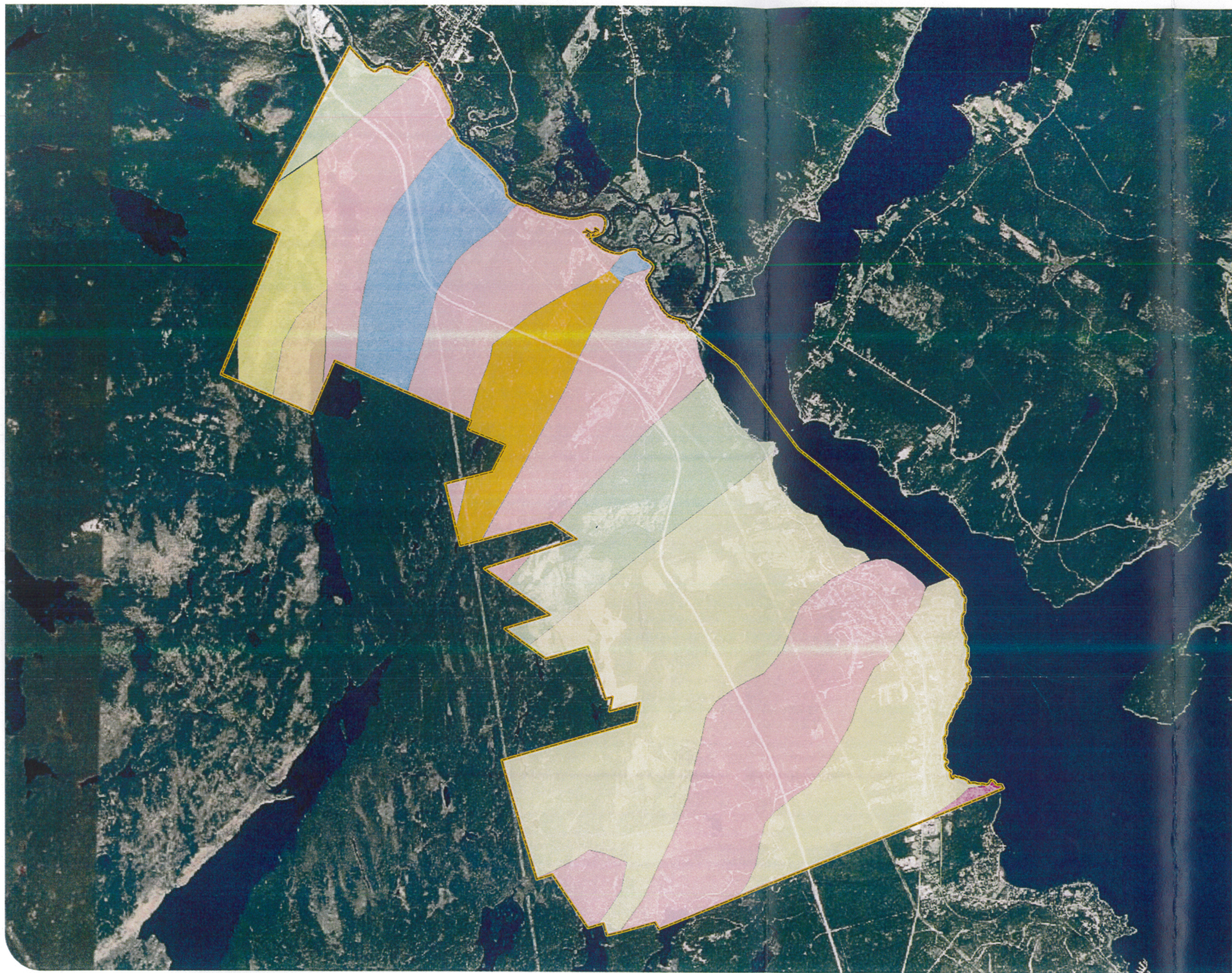
FIGURE 1 BEDROCK GEOLOGY
