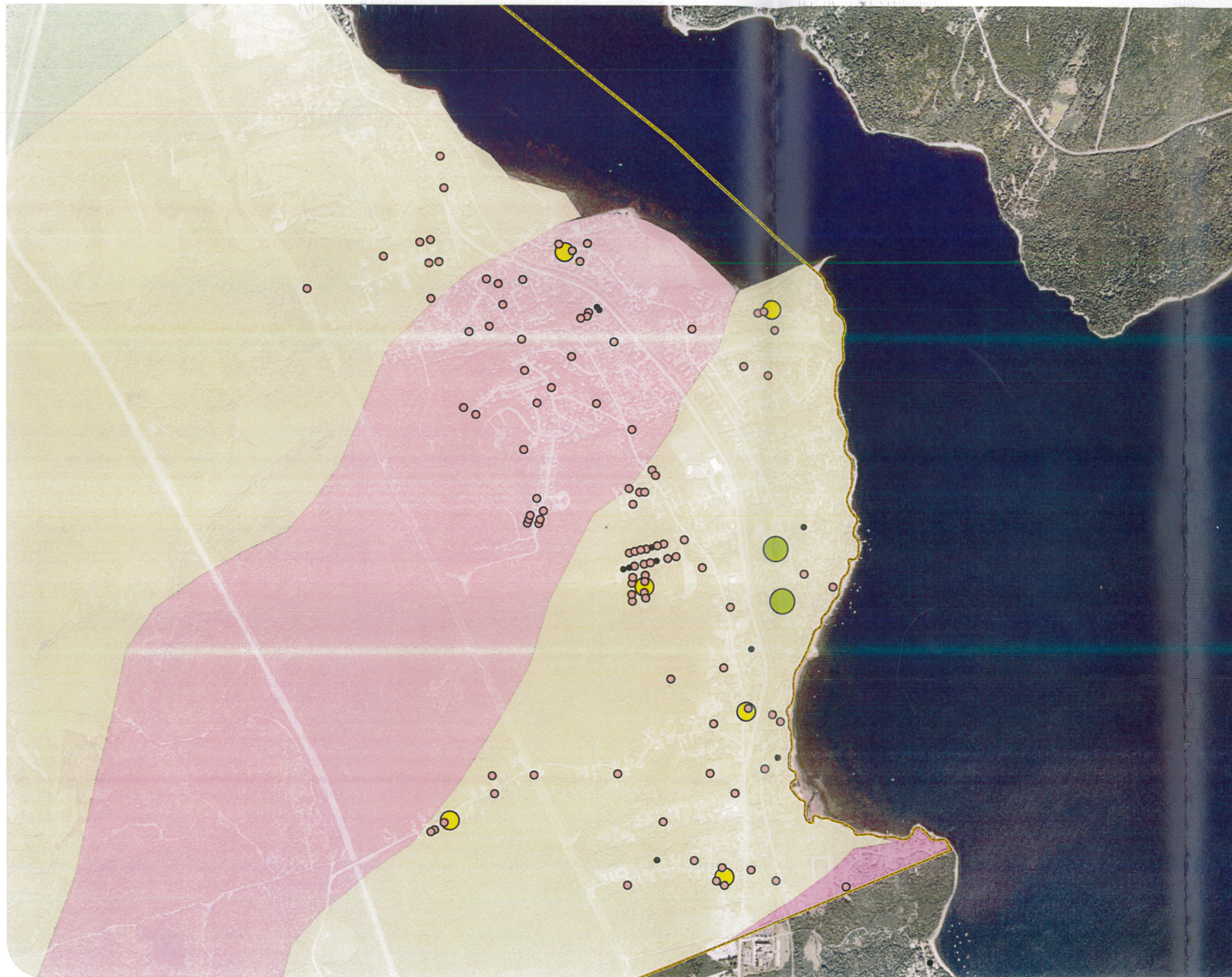
FIGURE 3B BEDROCK GEOLOGY AND WELL YIELDS
